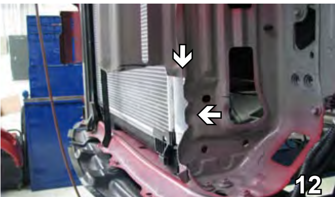
12. Showing the lower frame support webbing after the trimming has been completed.
