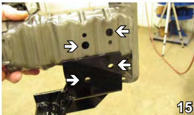
15. Line up the two big existing holes in the frame extension with the side baseplate holes. Start the 3/8 x 1 1/2" bolts. Do this on both sides.
